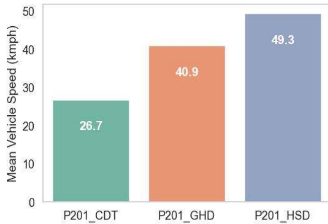
Mean Vehicle Speed Comparison
